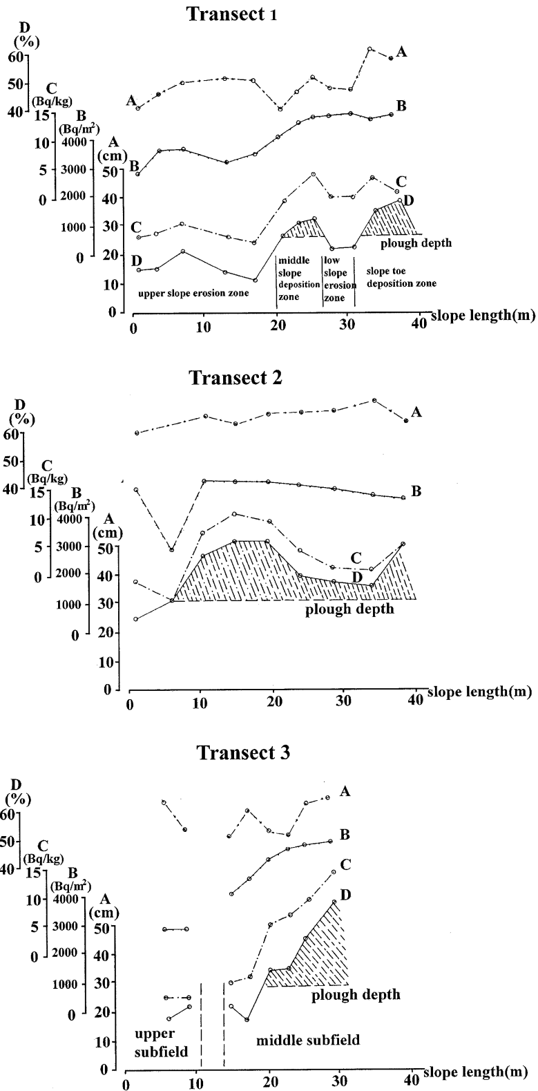
Figure 2. Variations 137 Cs distribution depth (A), 137 Cs inventory(B), and 137 Cs concentration(C) and percentage of >2 mm particles (D) along three transects.
