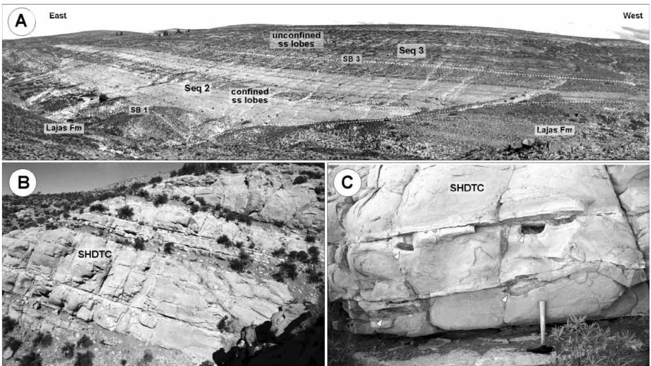
FIGURE 6 | A) Panoramic view of sequences 2 and 3 in the vicinity of section 7 (Los Catutos). Note the lenticular shape in large scale of the confined shelfal sandstone lobes of sequence 2 and the onlap above the Lajas Formation (on the right). B) Detail of thick massive sandstone beds deposited by long-lived sandy high-density turbidity currents in confined areas. See the geologist on the lower right corner for scale. C) Detail of massive sandstone beds with large floating clasts (arrows). Note their occurrence close to the bed top. SB: sequence boundary.
