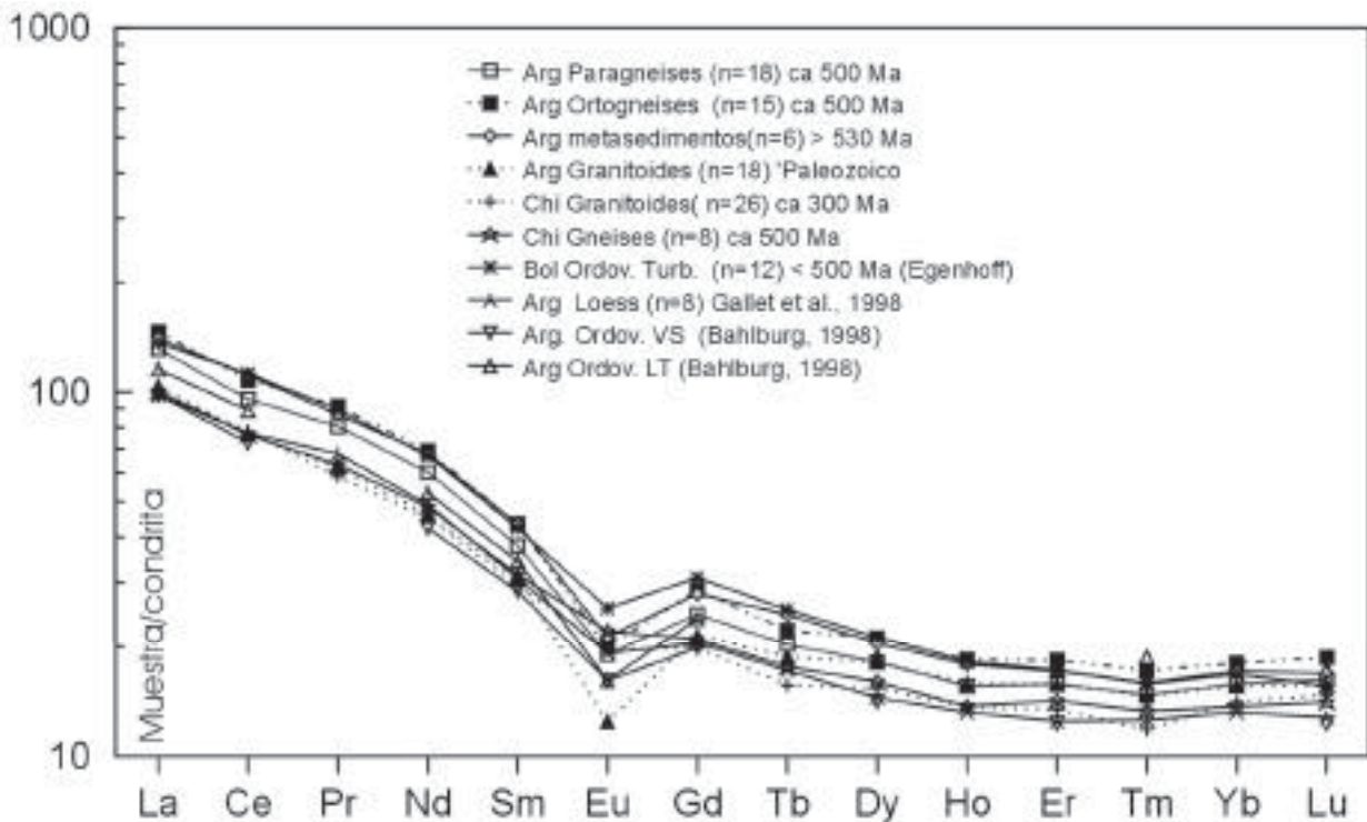
Figura 11. Average values of REE contents normalized to the C1 chondrite of various types of felsic rocks from NW-Argentina, northern Chile and southern Bolivia. Abbreviations: Bol. Ordov. Turb.: turbidites of Ordovician age of southern bolivia (Sven Egenhoff, TU-Berlin pers. comun.); Arg. Ordov. VS: volcano-sedimentary succession and Arg. Ordov. LT: turbidites of the lower sucession, both of Ordovician age from NW-Argentina (Bahlburg, 1998).
