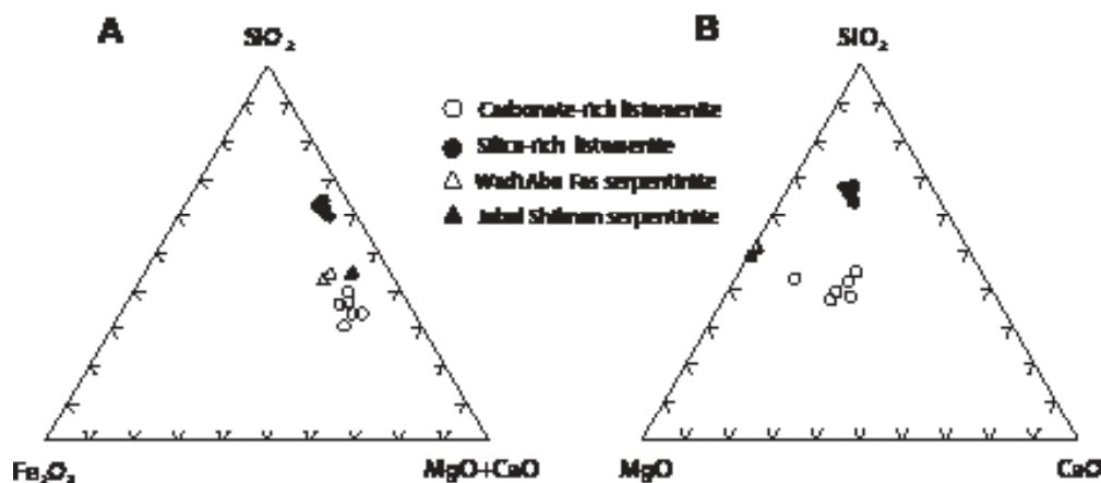
FIGURE 6 | Ternary diagrams for listwaenites and serpentinites (wt. %); A) SiO_2 - Fe_2O_3 - MgO+CaO , and B) SiO_2 - MgO - CaO diagrams. This diagram was first included in the literature by Uçurum (1996).
