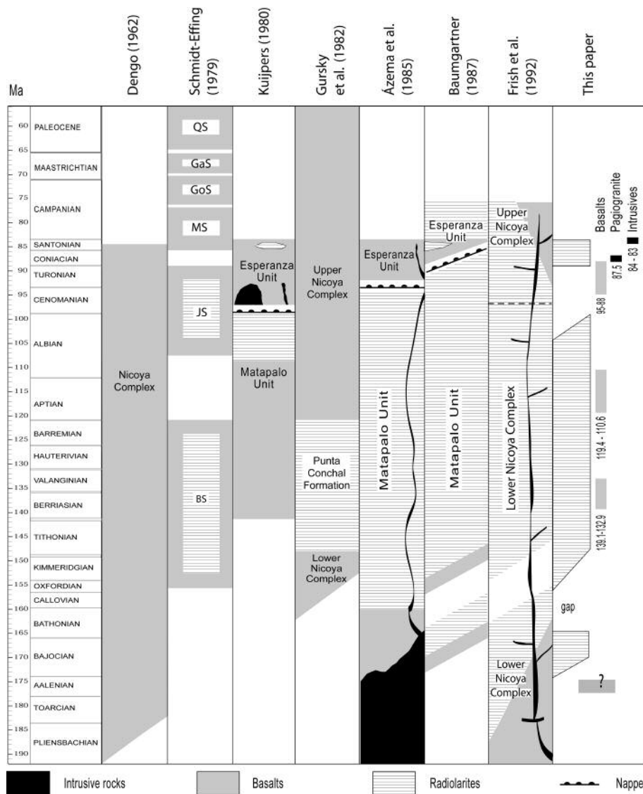
FIGURE 3 | Compared stratigraphic columns of the Nicoya Complex by different authors. BS: Brasilito Subcomplex; JS: Junquillo Subcomplex; MS: Murcielago Subcomplex; Go: Golfito Subcomplex; Ga: Garza Subcomplex; QS: Quepos Subcomplex. Time scale based on Channell et al., 1995; Gradstein et al., 1995, and Palfy et al., 2000.
