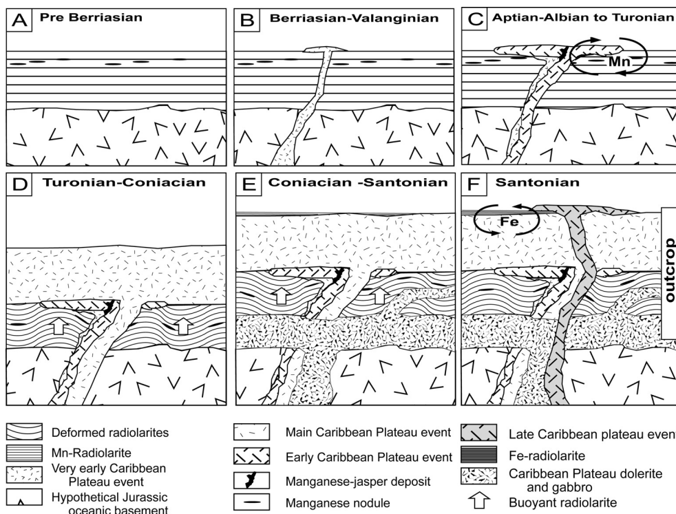
FIGURE 9 | Synopsis of Middle Jurassic to Late Cretaceous events that led to the formation of the Nicoya Complex drawn in schematic cross-sections (not to scale). We infer the emplacement of a plateau belonging to the CLIP (Caribbean Large Igneous Province) on a hypothetical Early to early Middle Jurassic oceanic crust, and “magmatic floating” of Jurassic-Cretaceous radiolarites.
