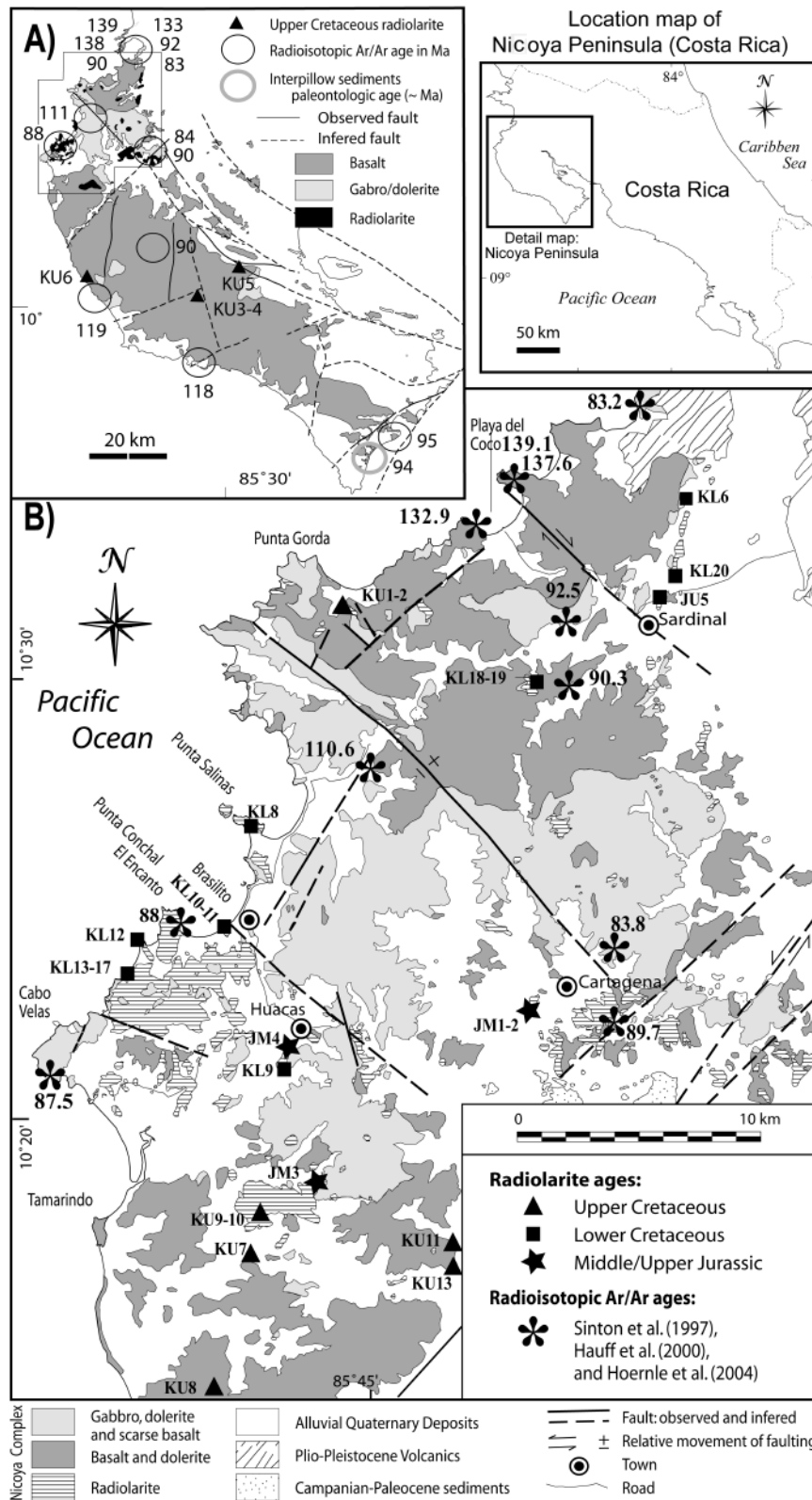
FIGURE 2 | A) Simplified Geologic map of the Nicoya Peninsula, with the location of the study area and other localities cited in the text. Based on Dengo (1962a), and unpublished data. B) Geologic map of the NW-Nicoya Peninsula after Denyer and Arias (1993), sample location of Middle Jurassic to Late Cretaceous radiolarian assemblages, and localities of Ar 39 /Ar 40 radioisotopic ages.
