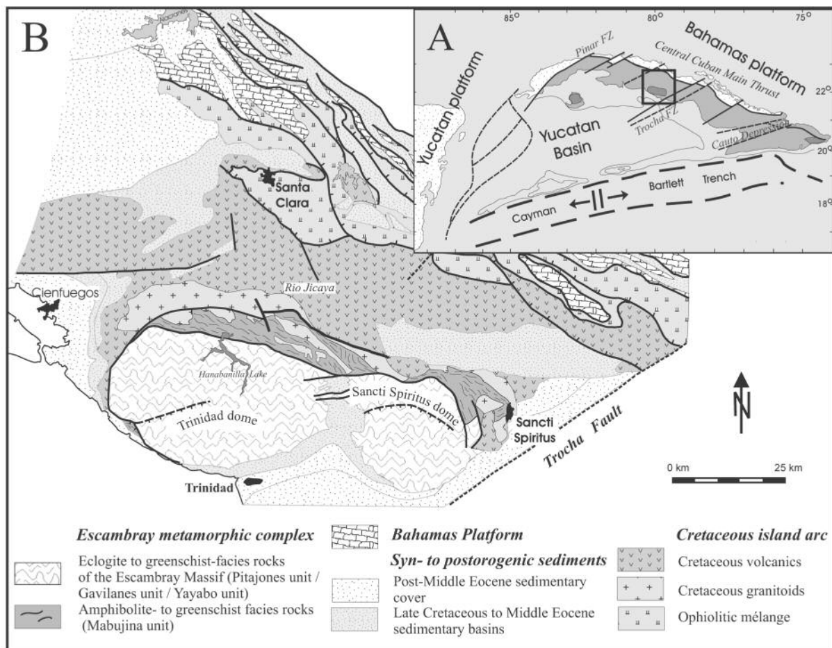
FIGURE 1 | A) Tectonic sketch of the Yucatán basin with the NCSZ and the position of the Escambray metamorphic complex. Light grey areas indicate the allochthonous island-arc sequences, dark grey areas the metamorphic complexes (Isla de la Juventud, Escambray, Sierra Purial from west to east). B) Overview of the geologic units of Las Villas (Central Cuba), modified after Stanek (2000).
