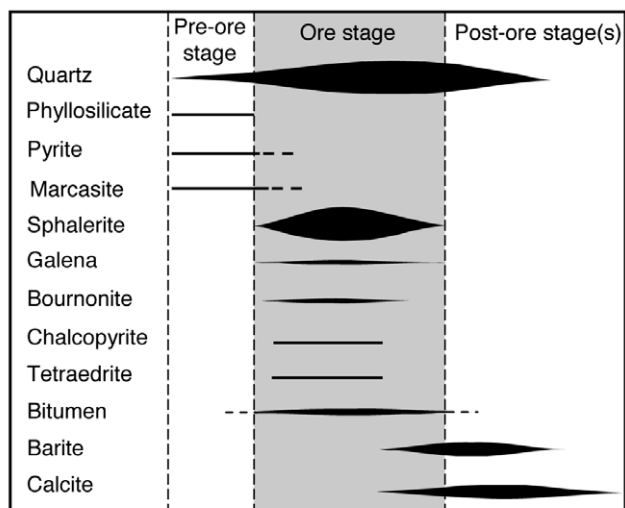
FIGURE 4 | Paragenetic sequence of the Itxaspe Zn-(Pb) mineralization.
