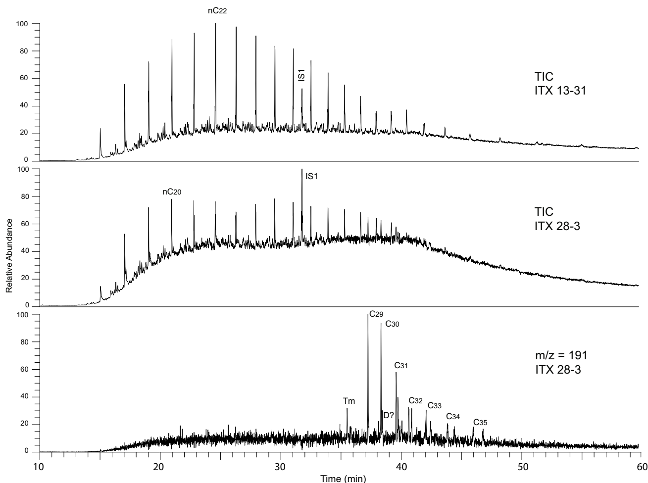
FIGURE 8 | Partially reconstructed chromatograms (TIC) of the saturated hydrocarbon fractions of samples ITX 13-31 and ITX 28-3 and distribution of hopanes in sample ITX 28-3, evidenced by selective m/z 191 ion detection. IS1 = internal standard (squalane). nC x = n-alkane. C x = regular hopane; D? = possible diahopane in C 29 .
