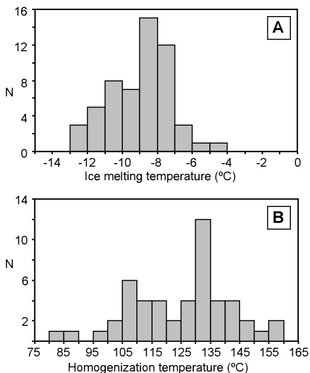
FIGURE 6 | A) Histogram of ice melting temperatures and B) histogram of homogenization temperatures of fluid inclusions in sphalerite from Itxaspe.
