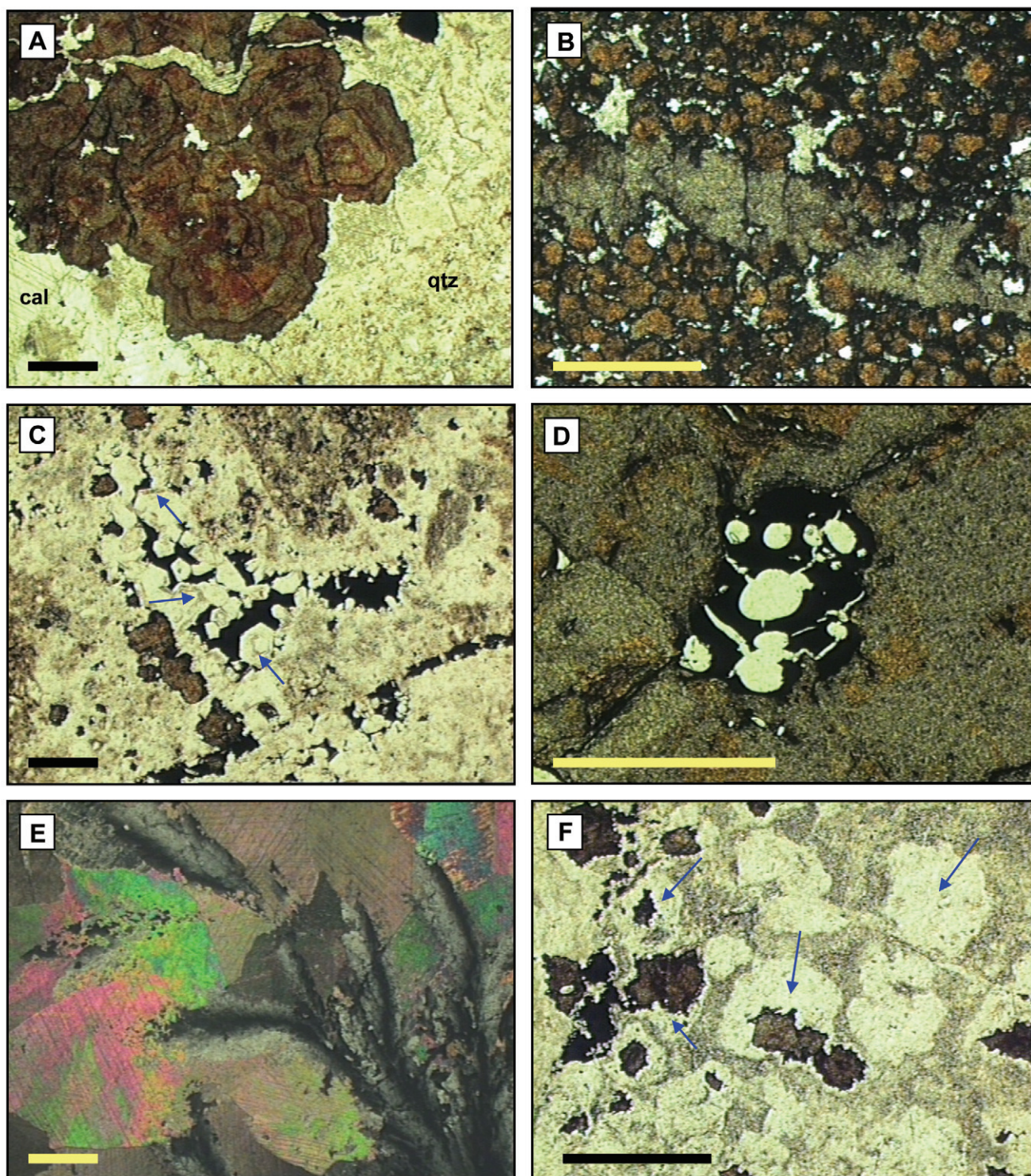
FIGURE 5 | Microscopic images under transmitted light. Scale bar is 500 µm. A ) Zoned, brown sphalerite, together with calcite (cal) and fine-grained quartz (qtz) (sample ITX16-2). B ) Brown sphalerite crystals crosscut by a late, honey-colored sphalerite vein (sample ITX20-1). C ) Sample with euhedral quartz crystals (central part) containing bitumen in growth bands (see arrows) and in contact with black solid bitumen patches (sample ITX16-7). D ) Black solid bitumen patch with degassing bubbles and contraction cracks, now filled with calcite. Brown phase is sphalerite (sample ITX13-3). E ) Barite crystals in fan-shaped aggregates (grey), together with calcite (sample ITX16-5). F ) Sphalerite (brown) and bournonite (black) crystals partially or completely replaced by late quartz (white). See arrows pointing to some of the replaced crystals. The matrix is made up of quartz and phyllosilicates (sample ITX16-2).
