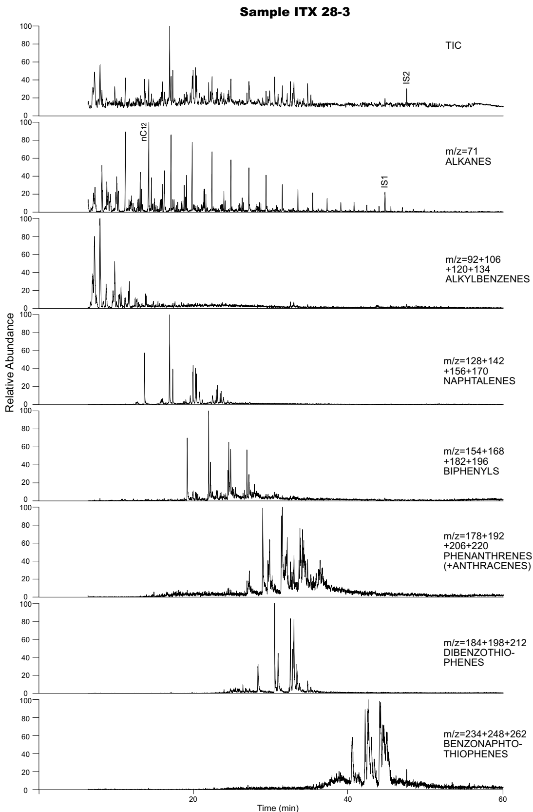
FIGURE 10 | Partially reconstructed chromatogram (TIC) of the on-line pyrolysate of sample ITX 28-3 and distribution of the major series of constituents recognized by selective ion detection. IS1 and IS2 = internal standards (squalane and \alpha -cholestane, respectively). nC_x = n-alkane.
