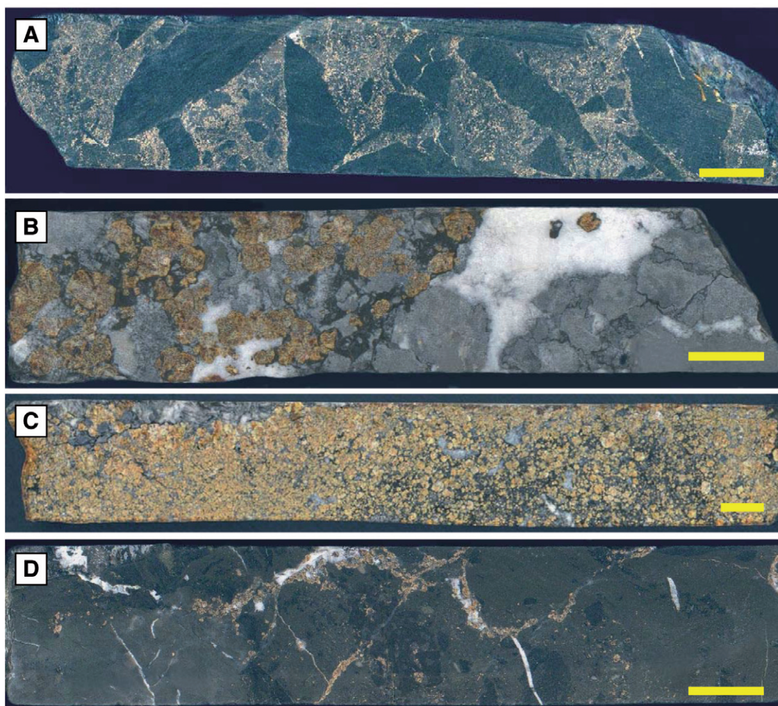
FIGURE 3 | Drill core samples of different host rocks and mineralization styles. Scale bar is 1 cm. A) Silicified breccia with disseminated sphalerite in the matrix (sample ITX13-1). B) White calcite and disseminated sphalerite replacing the limestone (sample ITX16-4). C) Massive sphalerite, with minor barite (grey) in the upper left part (sample ITX13-3). D) Silicified breccia with veinlets of sphalerite, calcite, barite and quartz (sample ITX16-6).
