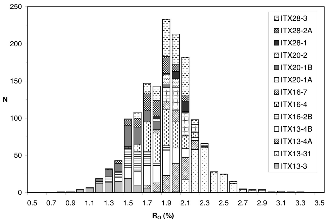
FIGURE 7 | Histogram of bitumen reflectivity data from Itxaspe.
