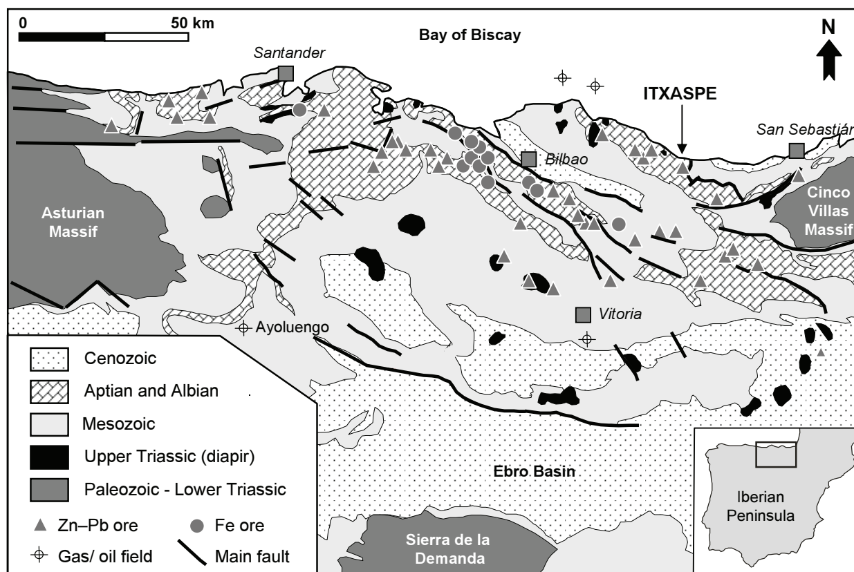
FIGURE 1 | Simplified geological map of the Basque-Cantabrian region (from García-Mondéjar et al., 1996), with the location of the Itxaspe Zn-(Pb) mineralization, of other Zn-Pb and Fe deposits and of oil and gas fields.
