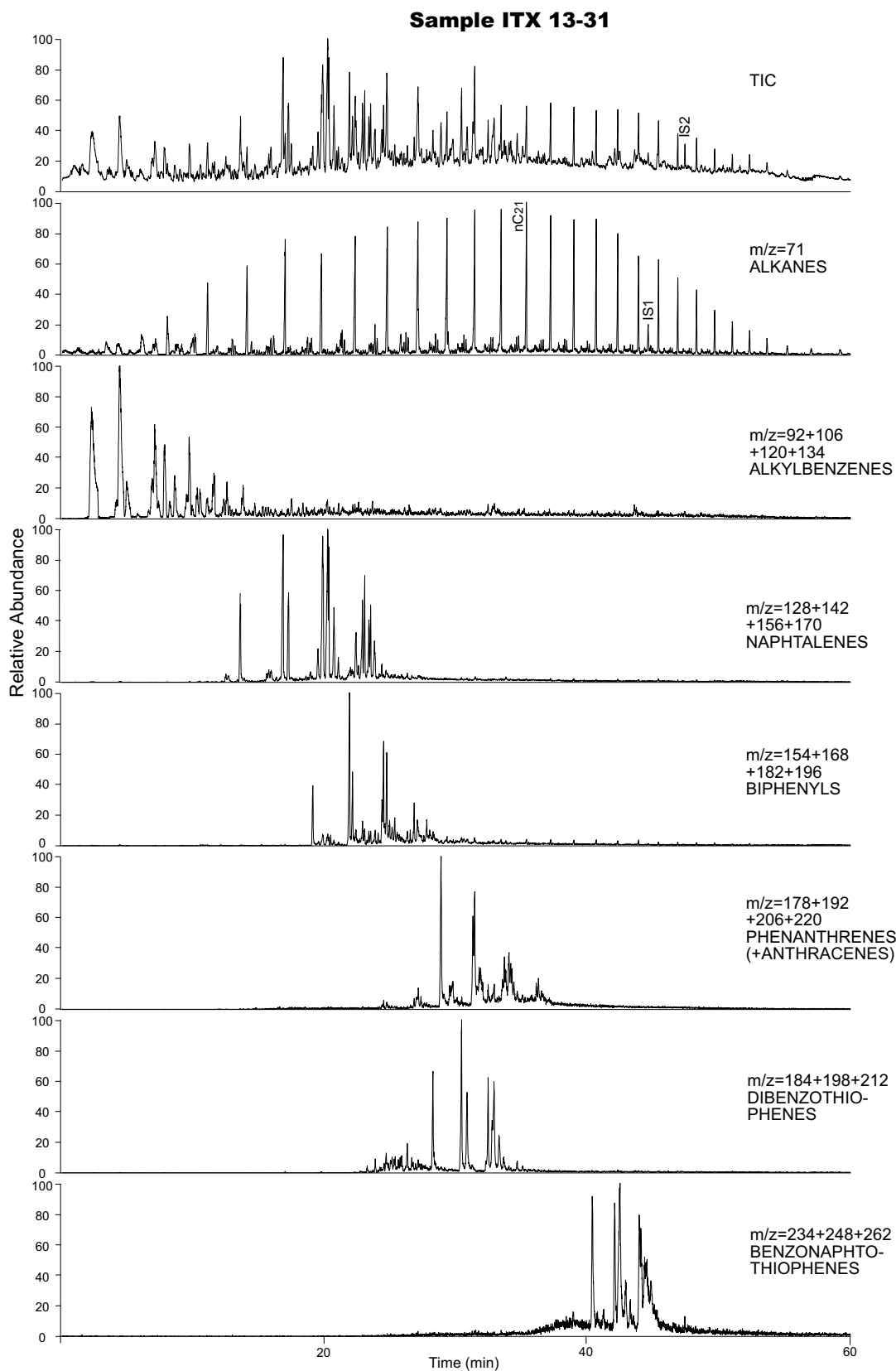
FIGURE 9 | Partially reconstructed chromatogram (TIC) of the on-line pyrolysate of sample ITX 13-31 and distribution of the major series of constituents recognized by selective ion detection. IS1 and IS2 = internal standards (squalane and \alpha -cholestane, respectively). nC_x = n-alkane.
