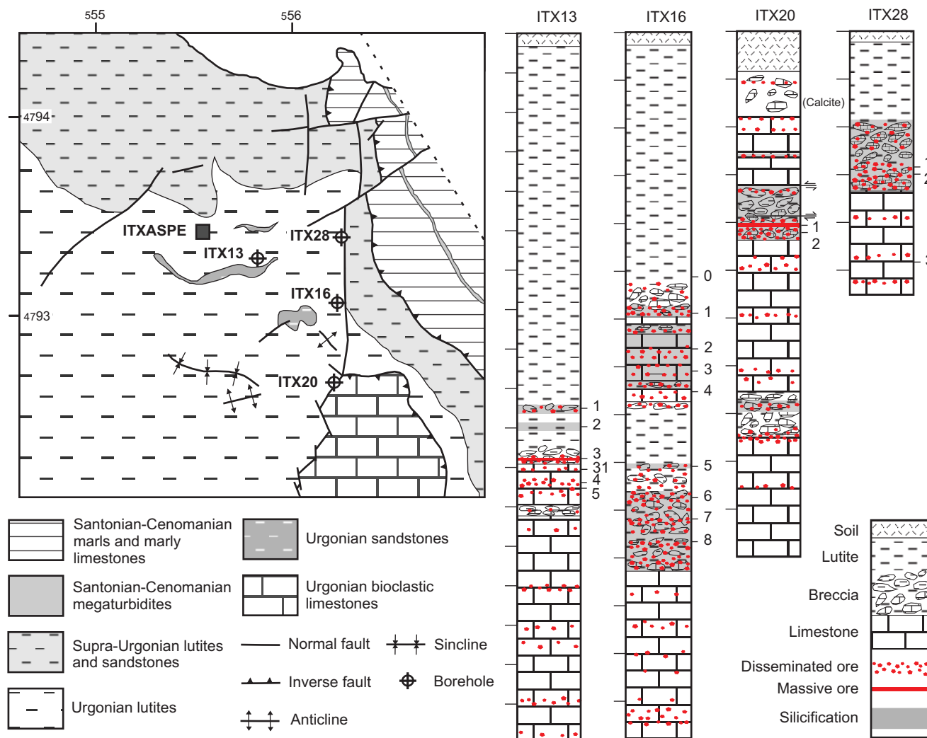
FIGURE 2 | Geological map of the area around Itxaspe (Outokumpu-EVE, 1995) with the locations of the sampled boreholes, and drill core description. Drill core vertical subdivisions are placed every 10 m. The position of the studied samples in the drill cores is also shown.
