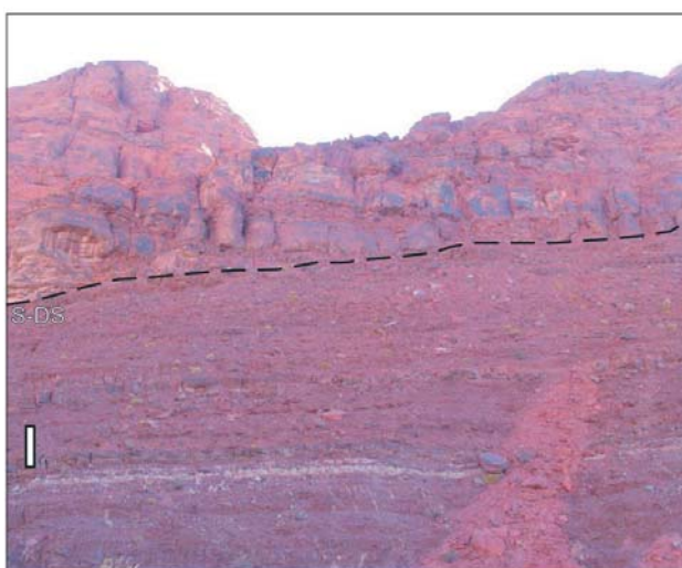
FIGURE 7 | Sand-drift surface (S-DS) separating playa lake deposits below from aeolian dune deposits above. The white bar is 1m thick.
