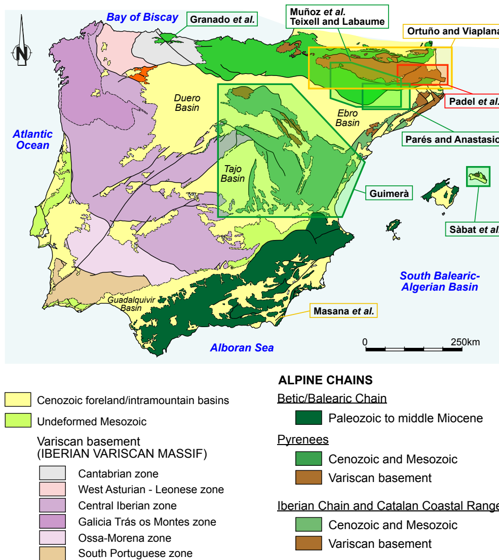
FIGURE 2. Major geological units of the Iberian Peninsula and Balearic Islands with setting of the contributions to this special volume.
