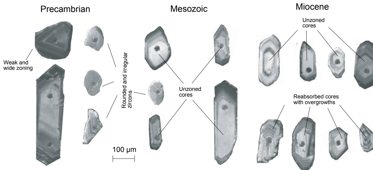
FIGURE 10. Cathodoluminescence (SEM-CL) images of selected LJS zircon grains discriminated by age ranges in the Precambrian, Mesozoic and Miocene. Black circles correspond to ablation pits from U/Pb dating.
