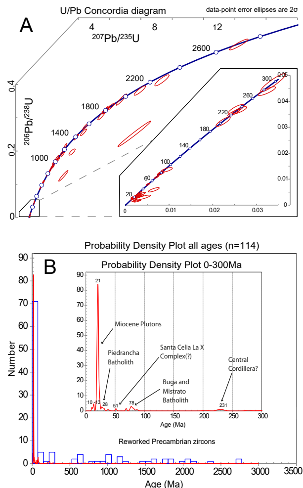
FIGURE 9. U/Pb results for 114 U/Pb dates reported in the detrital zircons for the LJSS sample. A) Concordia Diagram. B) Probability Density Plot (PDP). Larger PDP covers the entire age range reported. Smaller PDP covers ages between 0 and 300Ma where main peaks are marked with the names of some intrusive bodies of the Western Cordillera that fall in these intervals and that are considered as potential sources for detrital material.
