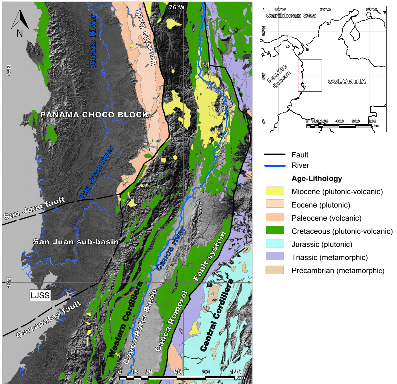
FIGURE 2. Main physiographic, structural, and chrono-stratigraphic framework (igneous and metamorphic units), adjacent to the Ladrilleros-Juanchaco Sedimentary Sequence (LJSS). Non-colored areas represent sedimentary rocks and Quaternary deposits. Modified from Gómez et al. (2015).
