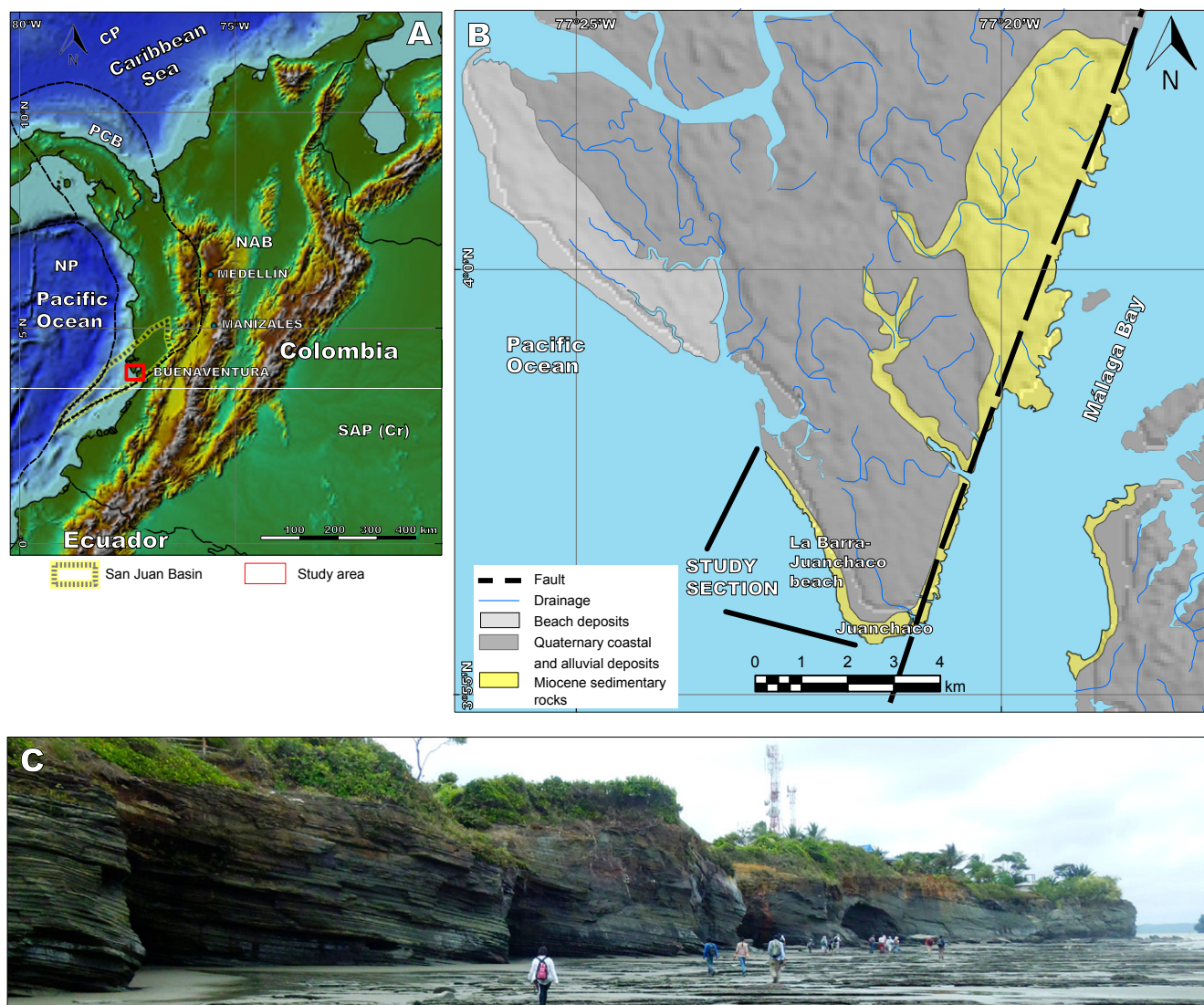
FIGURE 1. A) Location of the Ladrillos-Juanchaco Sedimentary Sequence (LJSS) on the Colombian and South American context on the Pacific coast. The general geodynamic setting is also shown with main tectonic plates and crustal blocks marked as CP: Caribbean Plate, NP: Nazca Plate, SAP-Cr: South American Plate and Craton, PCB: Panamá-Chocó Block, NAB: Nor-Andean Block (from Suter et al. , 2008; Taboada et al. , 2000; Cediel et al. , 2003). B) Local geological framework of the LJSS (modified from Montoya, 2003). C) General aspect of outcrops for the LJSS in the studied section, NW-SE.
