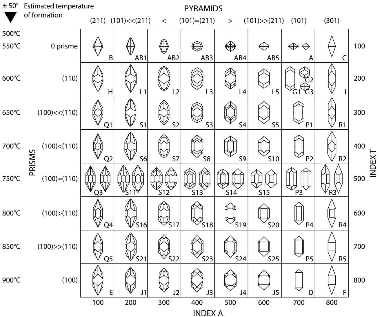
FIGURE 4. Zircon typological classification proposed by Pupin (1980). Index A reflects the Al/alkali ratio, controlling the development of pyramids in the crystals. Index T reflects the effects of temperature on the development of prisms.
