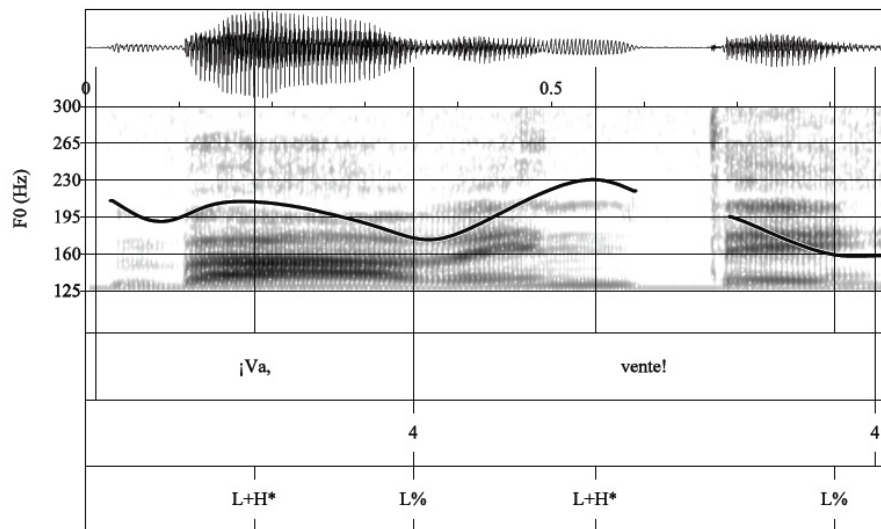
Figure 20. Waveform, spectrogram, and F0 trace for the request ¡Va, vente! ‘Come on, come [with us]!’ produced with a L+H* accent followed by a L% boundary tone.
