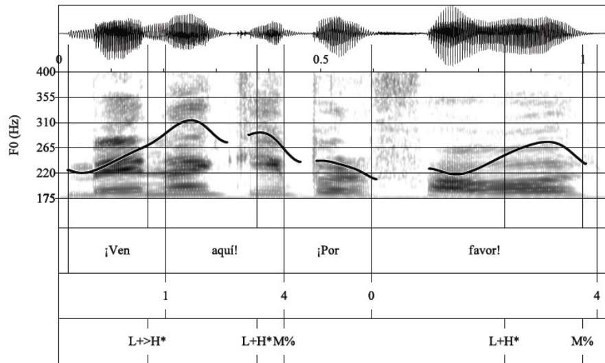
Figure 19. Waveform, spectrogram, and F0 trace for the command Ven aquí, por favor 'Come here, please' produced with a L+H* accent followed by a M% boundary tone.
