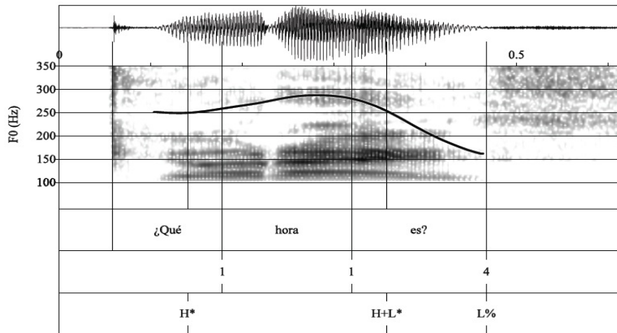
Figure 15. Waveform, spectrogram, and F0 trace for the information-seeking wh -question ¿Qué hora es? 'What time is it?' produced with a H+L* accent followed by a L% boundary tone.
