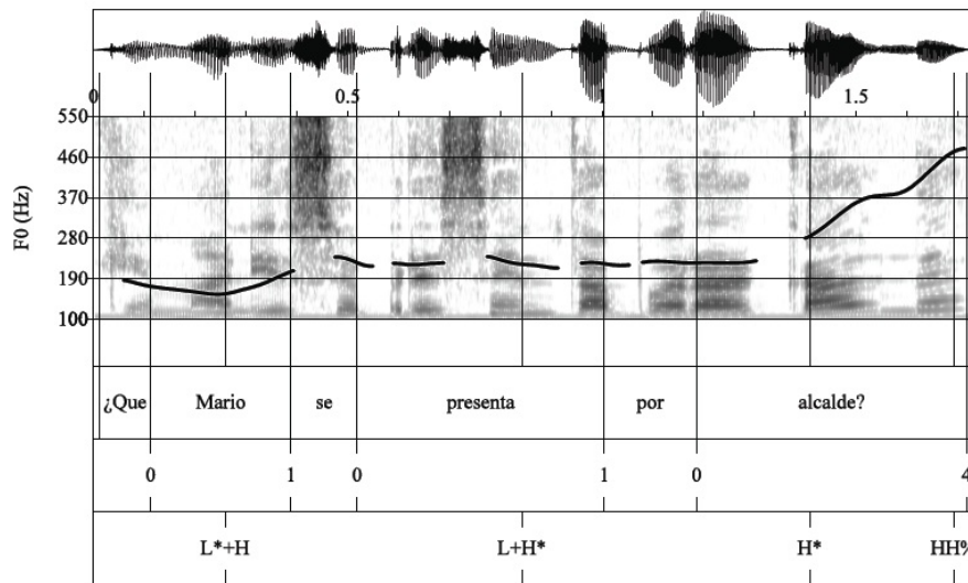
Figure 9. Waveform, spectrogram, and F0 trace for the counter-expectational yes/no question ¿Que Mario se presenta por alcalde? 'Mario is running for mayor?' produced with a H* nuclear accent followed by a HH% boundary tone.
