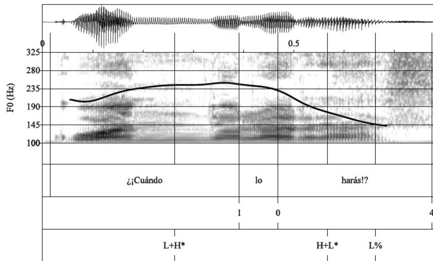
Figure 18. Waveform, spectrogram, and F0 trace for the imperative wh -question ¿Cuándo lo harás? ‘When are you going to do it?’ produced with a H+L* accent followed by a L% boundary tone.
