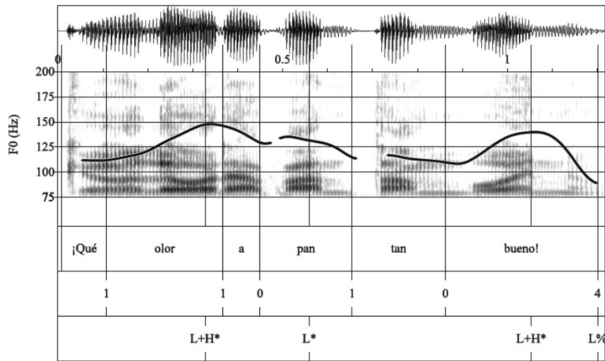
Figure 4. Waveform, spectrogram, and F0 trace for the exclamative statement ¡Qué olor a pan tan bueno! 'What a lovely aroma of bread!' produced with a L+H* nuclear accent followed by a L% boundary tone.
