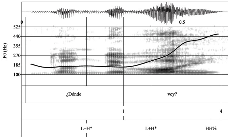
Figure 17. Waveform, spectrogram, and F0 trace for the echo wh-question ¿(Que) dónde voy? ‘[Did you ask me] where I’m going?’ produced with a L+H* accent followed by a HH% boundary tone.
