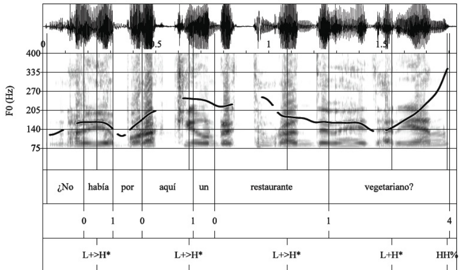
Figure 14. Waveform, spectrogram, and F0 trace for the yes/no outer negation question ¿No había por aquí un restaurante vegetariano? 'Wasn't there a vegetarian restaurant around here?' produced with a L+H^* accent followed by a HH\% boundary tone.
