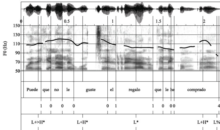
Figure 6. Waveform, spectrogram, and F0 trace for the uncertainty statement Puede que no le guste el regalo que le he comprado ‘ S/he may not like the present that I have bought him/her ’ produced with a L+H* nuclear accent followed by a L% boundary tone.
