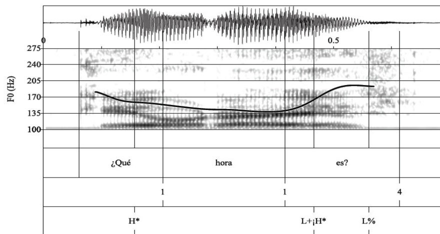
Figure 16. Waveform, spectrogram, and F0 trace for the information-seeking wh -question ¿Qué hora es? 'What time is it?' produced with a L+¡H* accent followed by a L% boundary tone.
