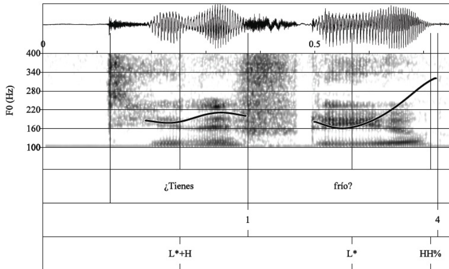
Figure 11. Waveform, spectrogram, and F0 trace for the yes/no confirmation question ¿Tienes frío? 'Are you cold?' produced with a L^* nuclear accent followed by a HH\% boundary tone.
