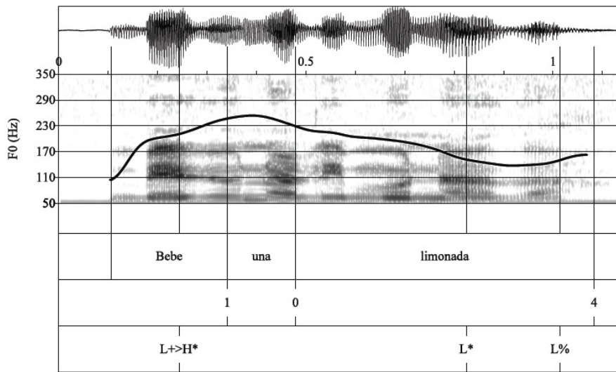
Figure 1. Waveform, spectrogram, and F0 trace for the broad focus statement Bebe una limonada 'S/he drinks a lemonade' produced with a L+>H^* prenuclear accent and L^* nuclear accent followed by a L\% boundary tone.
