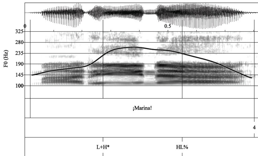
Figure 22. Waveform, spectrogram, and F0 trace for the insistent vocative contour ¡Marina! ‘Marina!’ produced with a L+H* accent followed by the bitonal HL% boundary tone.
