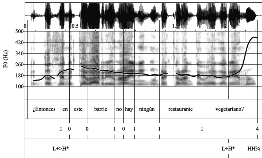
Figure 13. Waveform, spectrogram, and F0 trace for the yes/no inner negation question ¿Entonces en este barrio no hay ningún restaurante vegetariano? ‘Then in this neighborhood there is no vegetarian restaurant?’ produced with a L+H* accent followed by a HH% boundary tone.
