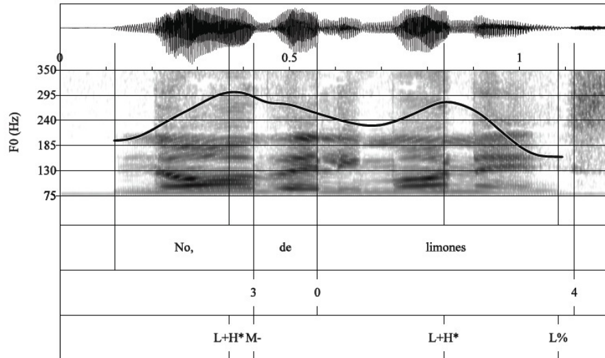
Figure 2. Waveform, spectrogram, and F0 trace for the narrow focus correction statement No, de limones 'No, of lemons' produced with a L+H* nuclear accent followed by a L% boundary tone.
