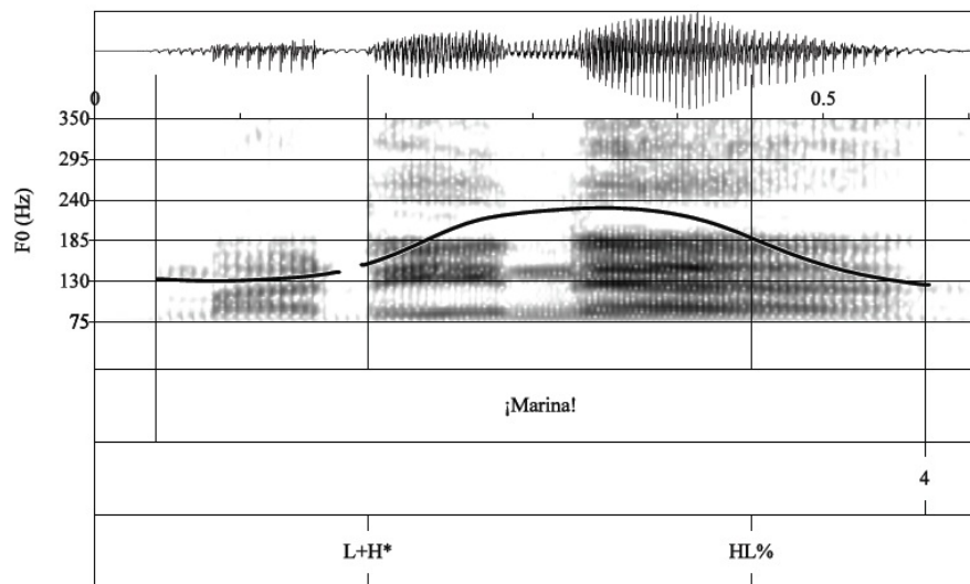
Figure 21. Waveform, spectrogram, and F0 trace for the vocative calling contour ¡Marina! ‘Marina!’ produced with a L+H* accent followed by the bitonal HL% boundary tone.
