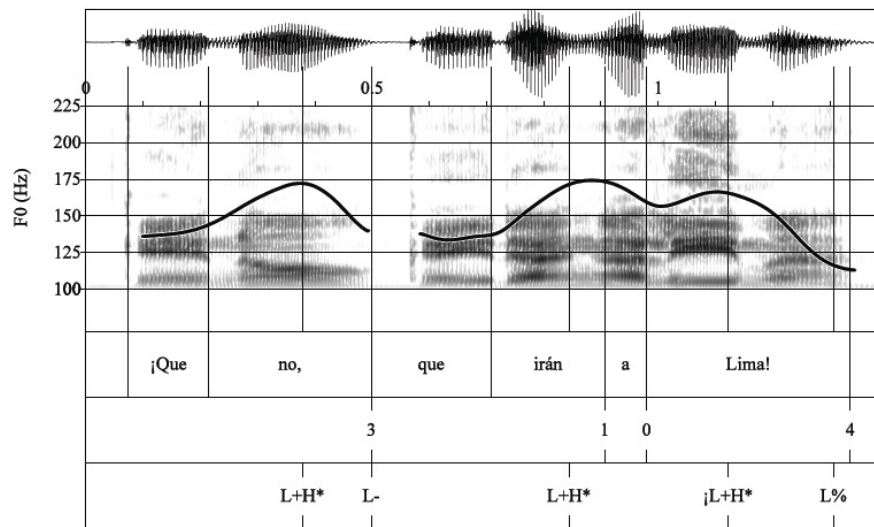
Figure 3. Waveform, spectrogram, and F0 trace for the narrow focus contradiction statement ¡Que irán a Lima! ‘They are going to Lima!’ produced with a ¡L+H* nuclear accent followed by a L% boundary tone.
