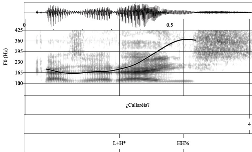
Figure 10. Waveform, spectrogram, and F0 trace for the imperative yes/no question ¿Callaréis? ‘Will you be quiet?’ produced with a L+H* nuclear accent followed by a HH% boundary tone.
