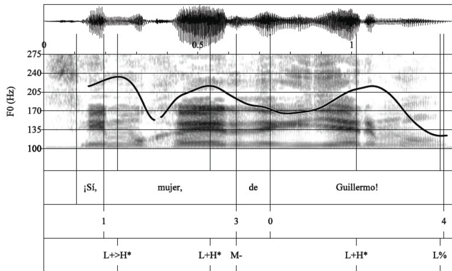
Figure 5. Waveform, spectrogram, and F0 trace for the statement of the obvious ¡Sí, mujer, de Guillermo! 'Yes, woman, Guillermo's [of course]!' produced with a L+H* nuclear accent followed by a L% boundary tone.
