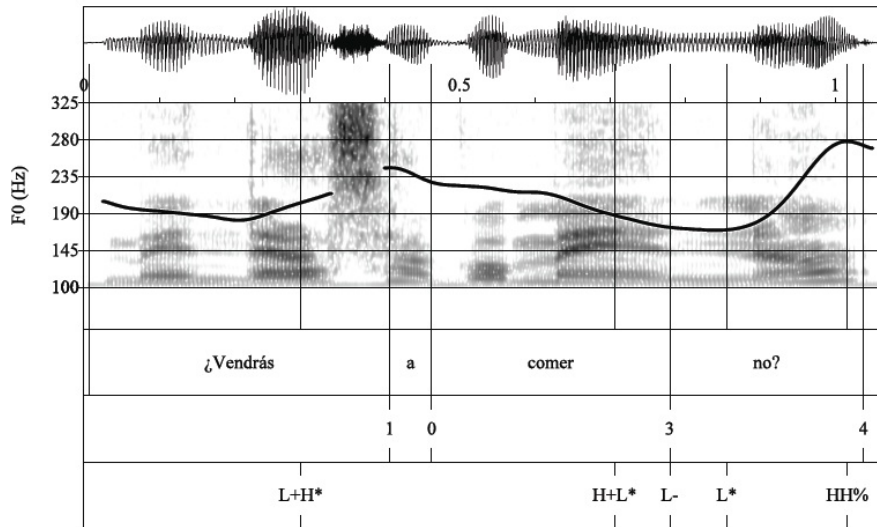
Figure 12. Waveform, spectrogram, and F0 trace for the yes/no tag question ¿Vendrás a comer, no? 'You'll come to eat, right?' produced with a L^* accent followed by a HH\% boundary tone.
