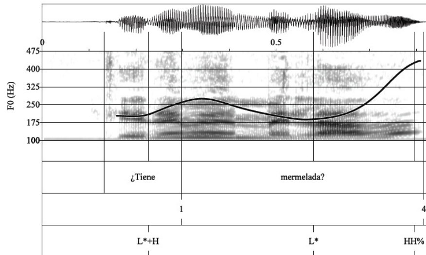
Figure 7. Waveform, spectrogram, and F0 trace for the information-seeking yes/no question ¿Tiene mermelada? 'Do you have any jam?' produced with a L^* nuclear accent followed by a HH\% boundary tone.
