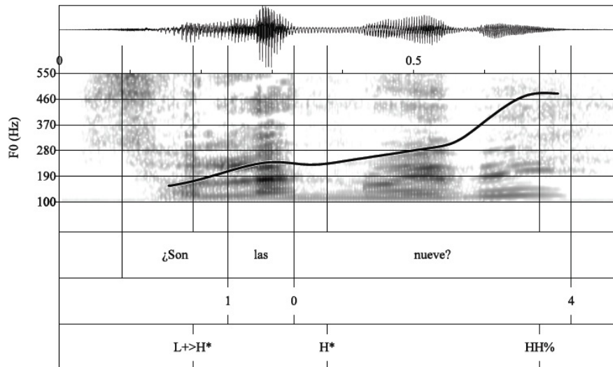
Figure 8. Waveform, spectrogram, and F0 trace for the echo yes/no question ¿(Que) son las nueve? ‘(Are you saying) that it’s nine o’clock?’ produced with a H* nuclear accent followed by a HH% boundary tone.
